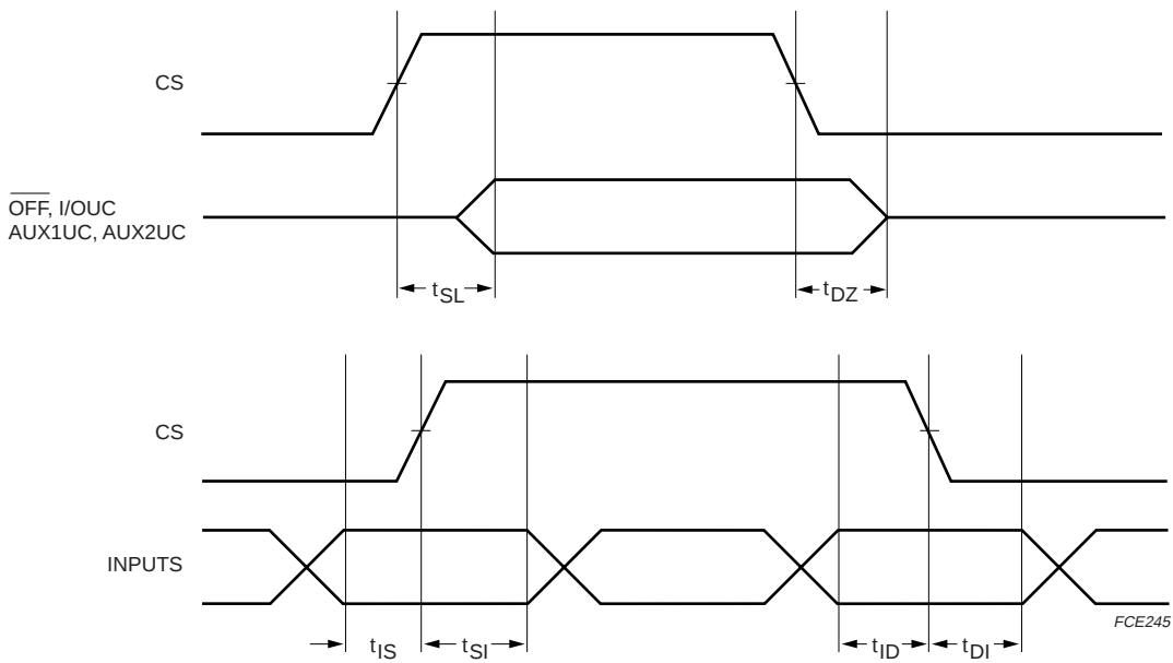
Fig.7 Chip select.
