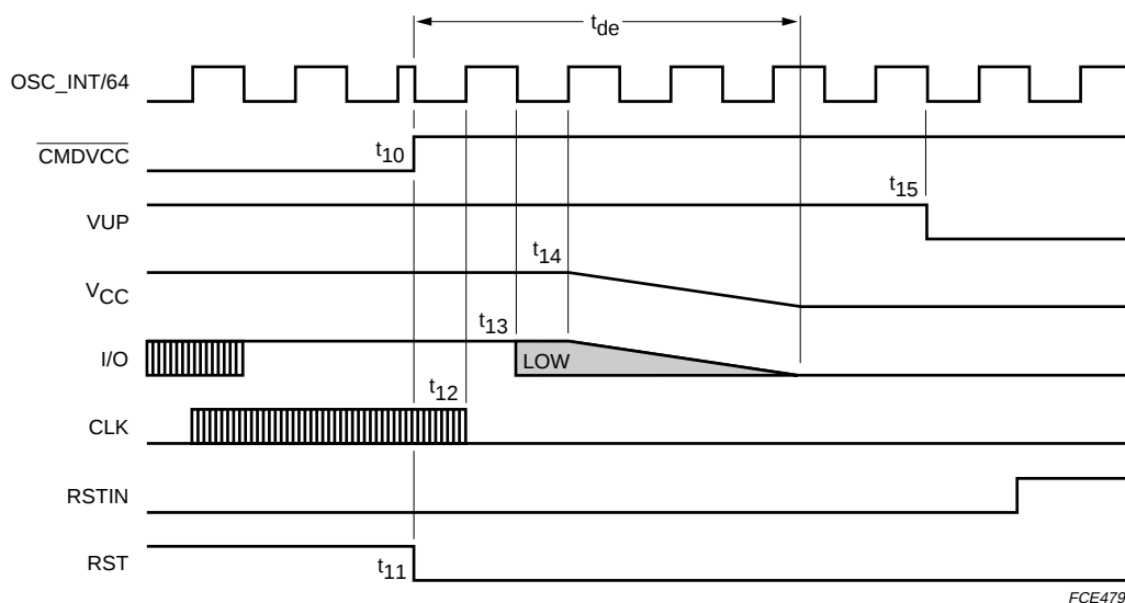
Fig.13 Deactivation sequence
